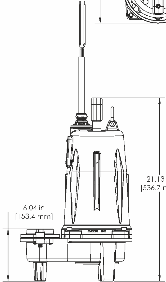
LEH200M3-E SERIES LEH150M2-E SERIES 2" FNPT DISCHARGE FLANGE
